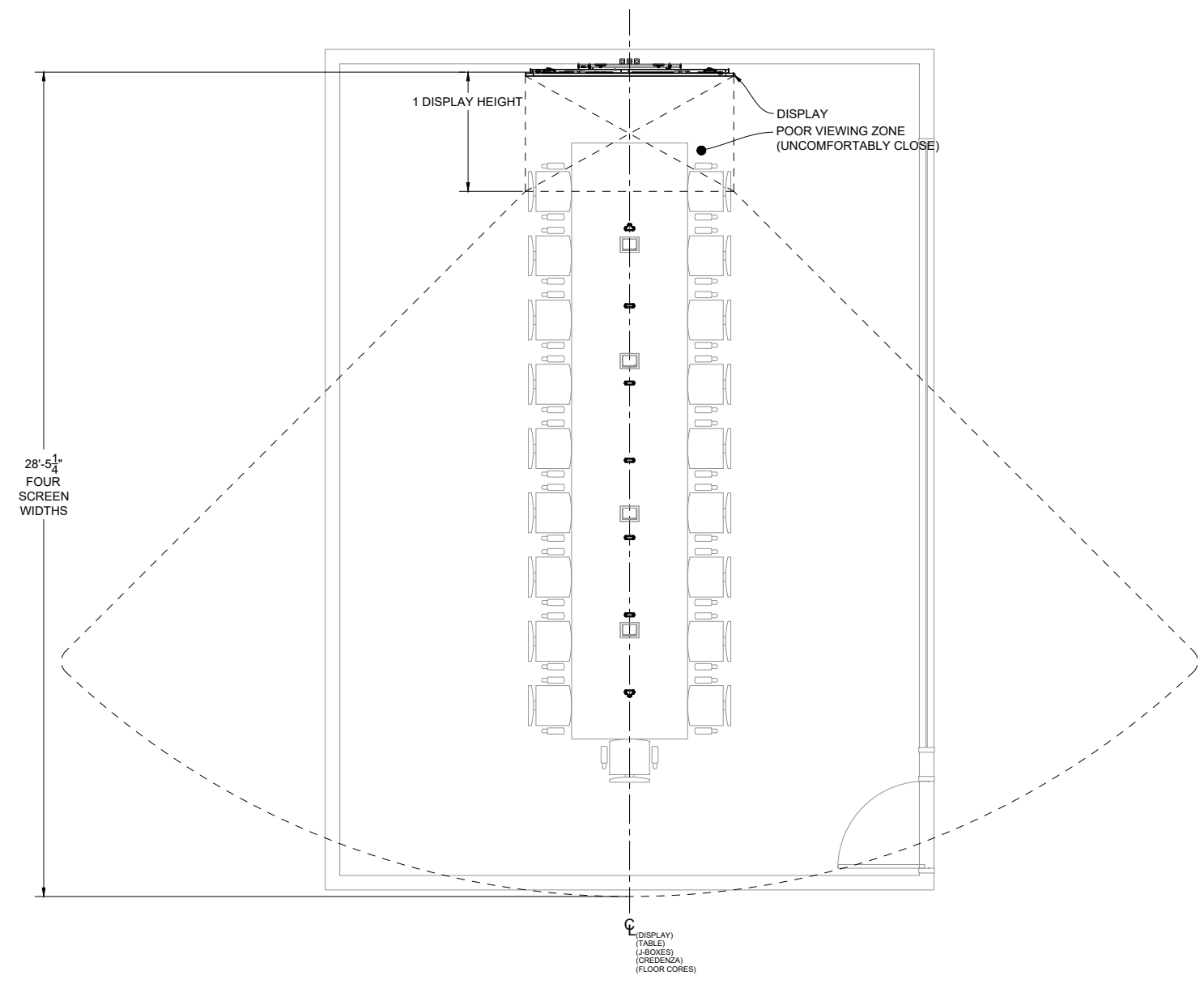
2 98" DISPLAY VIEWERSHIP - PLAN DNADT-02 SCALE: 3/16" = 1'-0"
